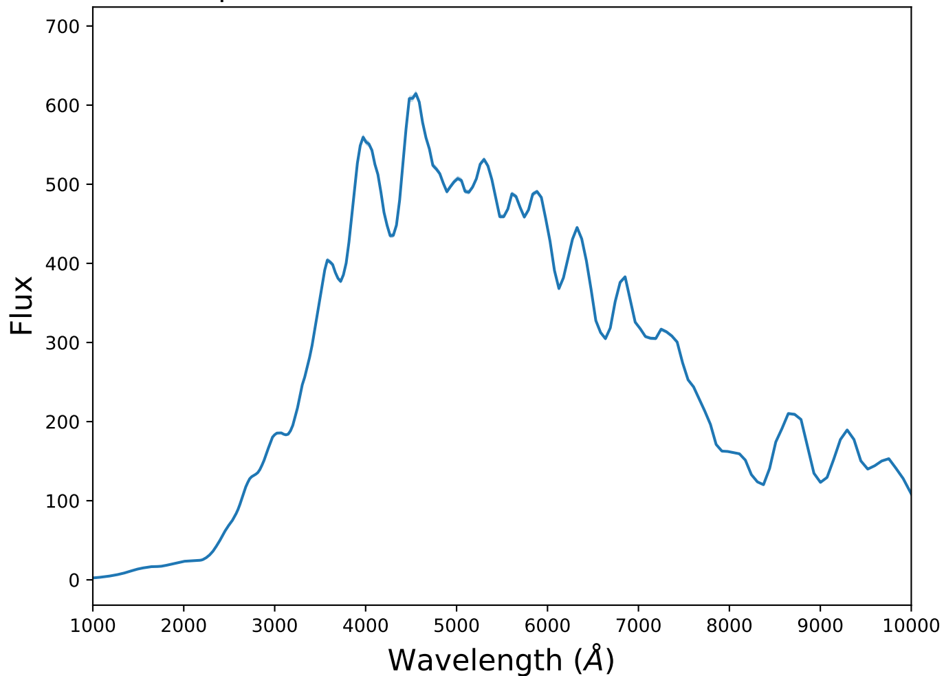
Spectrum 3 for transient CCSN at z=0.26
